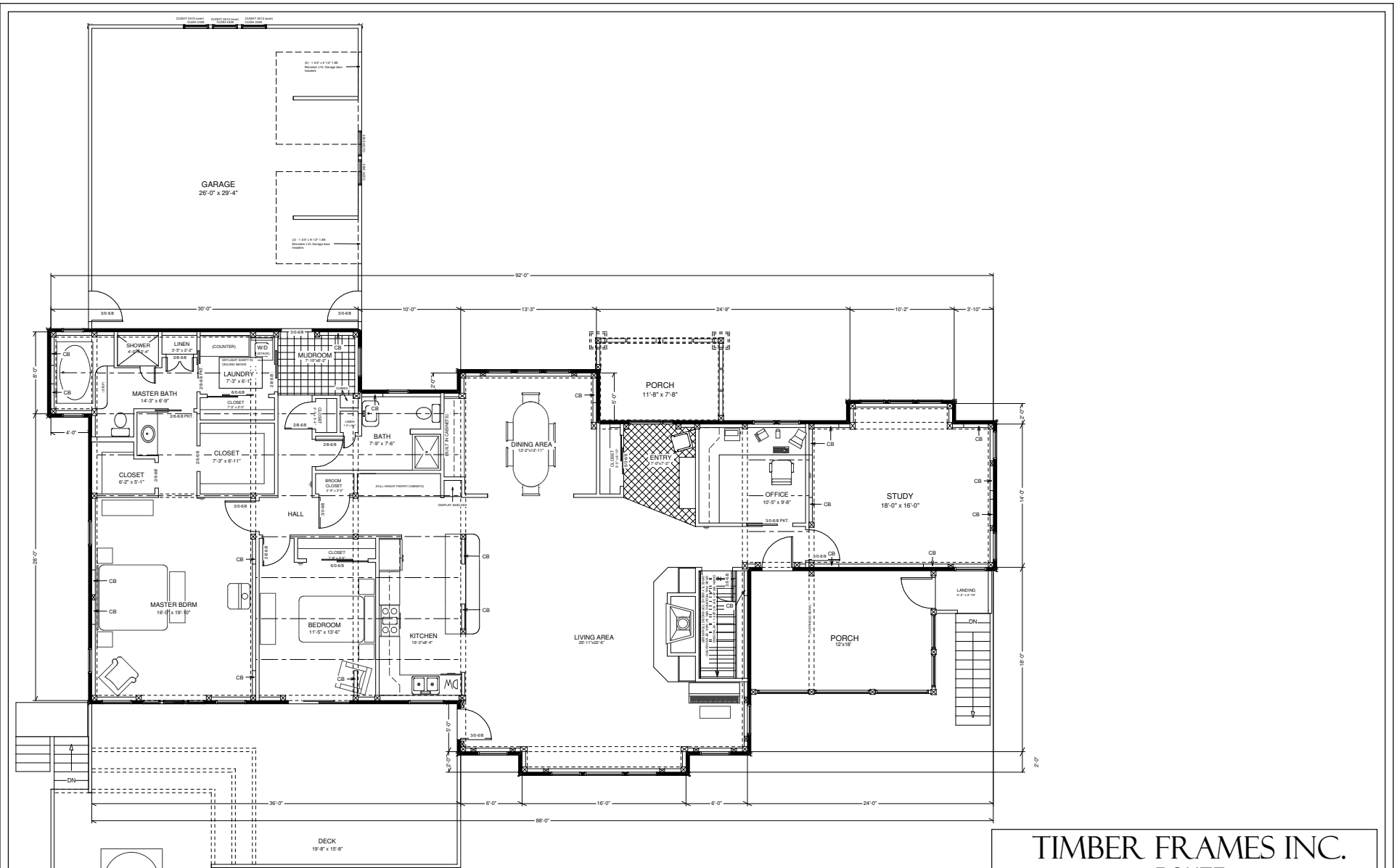
FLOOR PLAN
