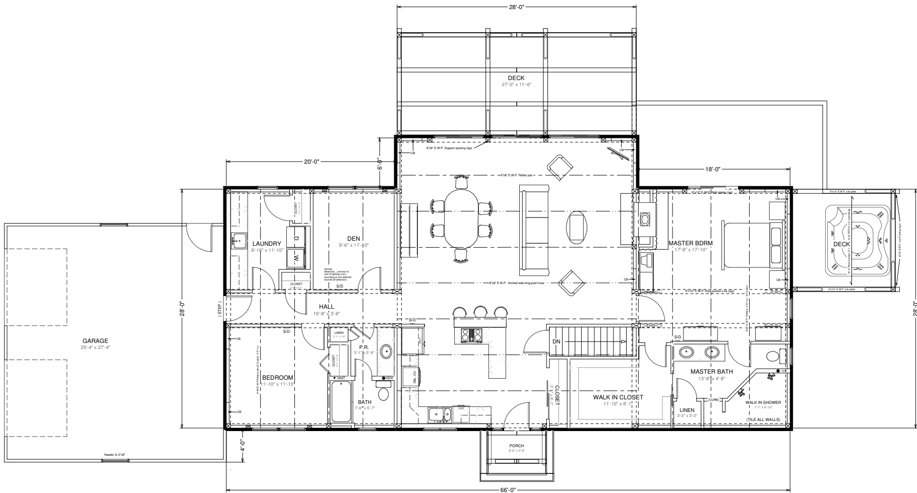
FLOOR PLAN
